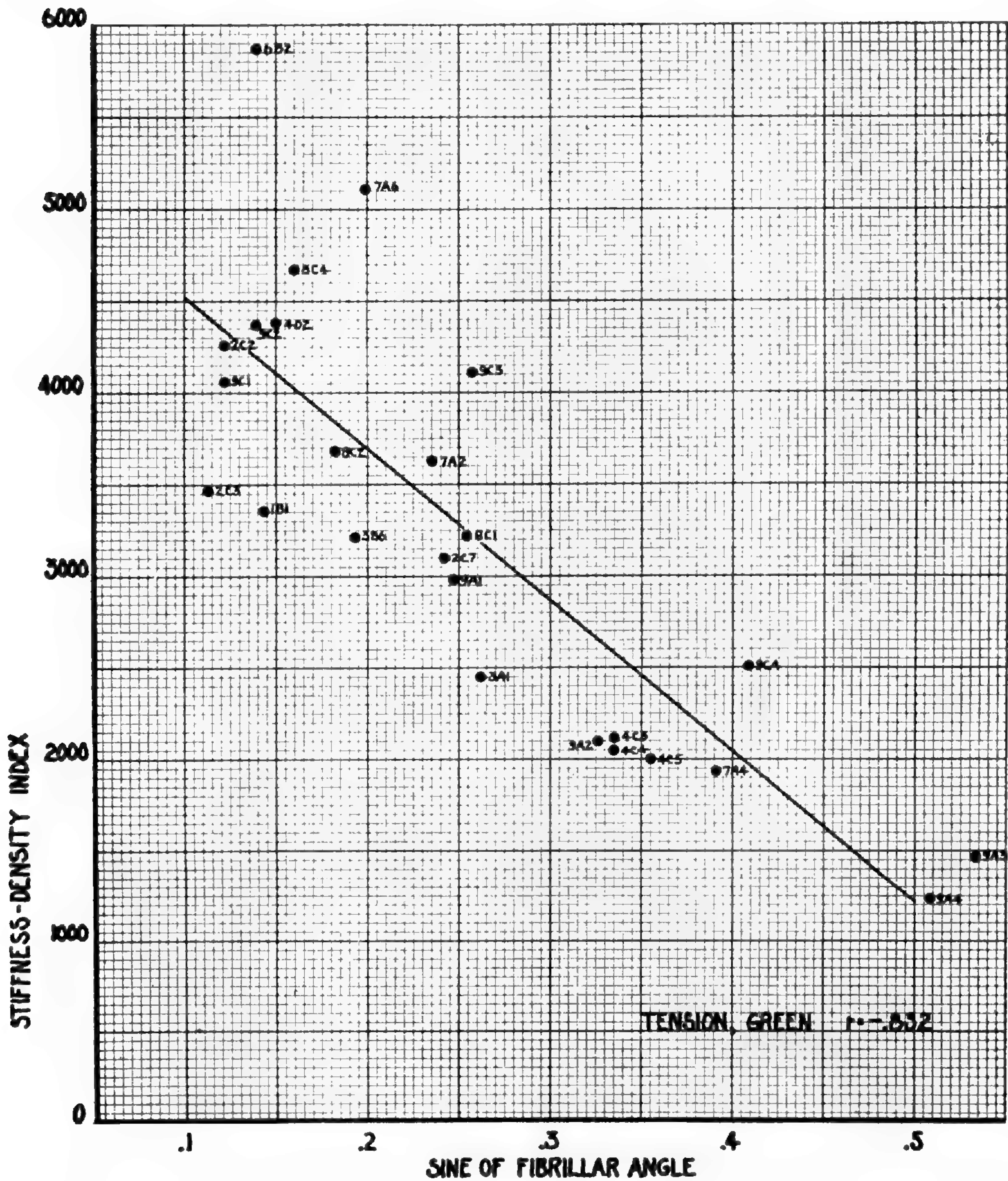
Fig. 11. Axial tension stiffness-density index (modulus of elasticity \div specific gravity) correlated with sine of average fibrillar angle in summerwood for green specimens.
